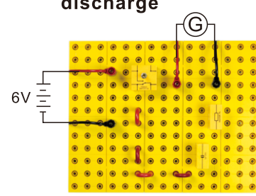
Capacitor charge and discharge
