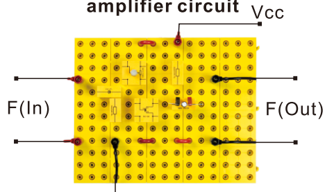
Basic transistor amplifier circuit
