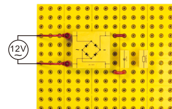
Capacitor charge and discharge
